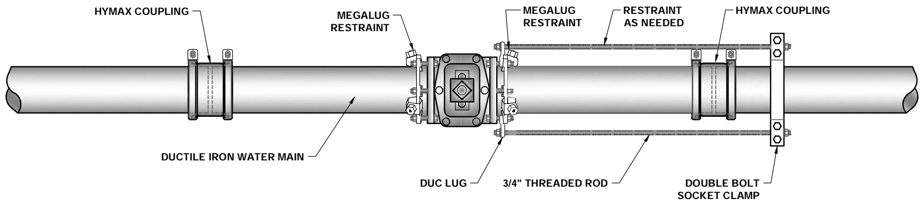
TYPICAL GATE VALVE W/ HYMAX COUPLINGS NOT TO SCALE
